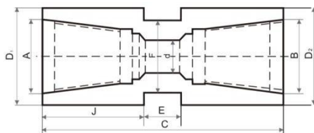
Box-Box Adapters
