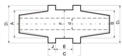
Pin-Pin Adapters
