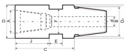
Pin-Box Adapters
